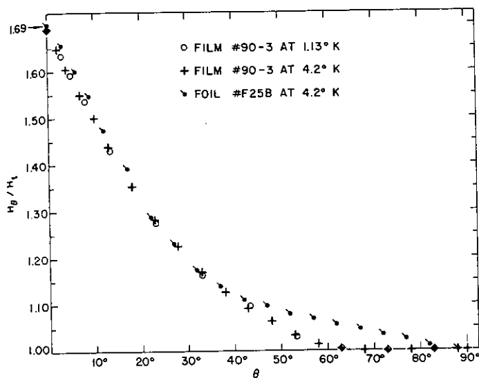
Figure 6. Ratio of transition field ( H_0 ) to transition field ( H_t ) for \theta = \frac{\pi}{2} versus \theta (angle between magnetic field and plane of film) for thick Pb-Tl films. The ratio 1.69 for \theta = 0 matches exactly the theoretical prediction for the superconducting sheath. (After Tomasch and Joseph, 1964.)
