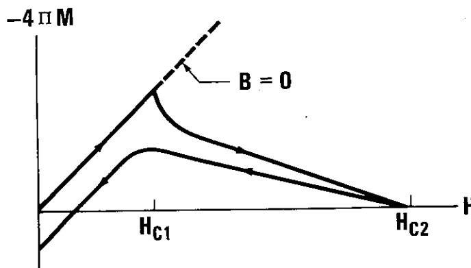
Figure 1. Magnetization (M) versus magnetic field (H) for typical non-ideal type II superconductor.
