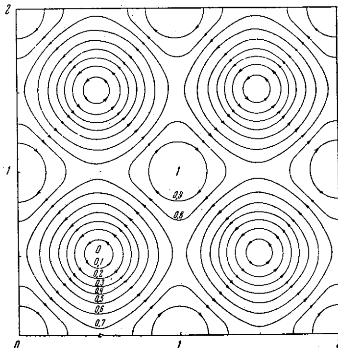
Figure 3. The Abrikosov vortex lattice.
