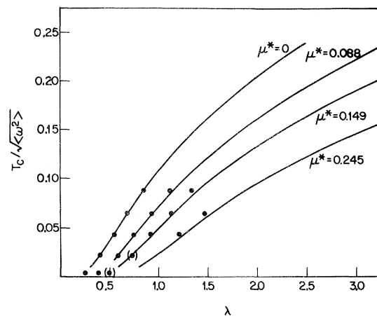
FIG. 4. T_c/(\langle \omega^2 \rangle)^{1/2} plotted versus \lambda . The solid lines are calculated from Eq. (14) using N=63 , for various values of \mu^* and the same shape \alpha^2 F(\omega) as used by McMillan to represent niobium. The points are McMillan's calculations as summarized in Table I of Ref. 1. The points enclosed in parentheses have \mu^* = 0.157 , otherwise \mu^* is the same as on the nearest labeled line. The agreement between these independent calculations is excellent except for a systematic deviation for large \mu^* , which probably derives from a slight difference in the definition of \mu^* , which is unimportant if \mu^* is small.
