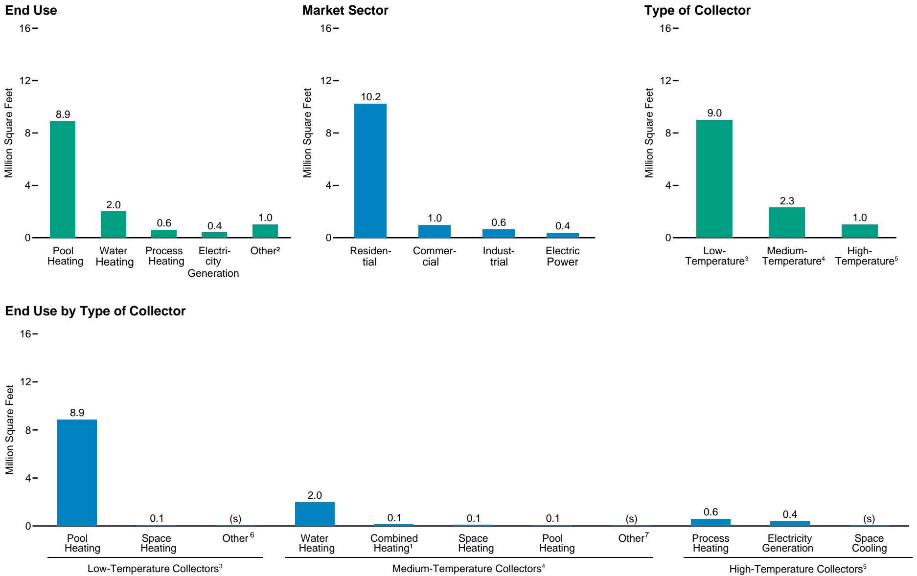
Figure 10.7 Solar Thermal Collector Domestic Shipments by Market Sector, End-Use, and Type, 2009
