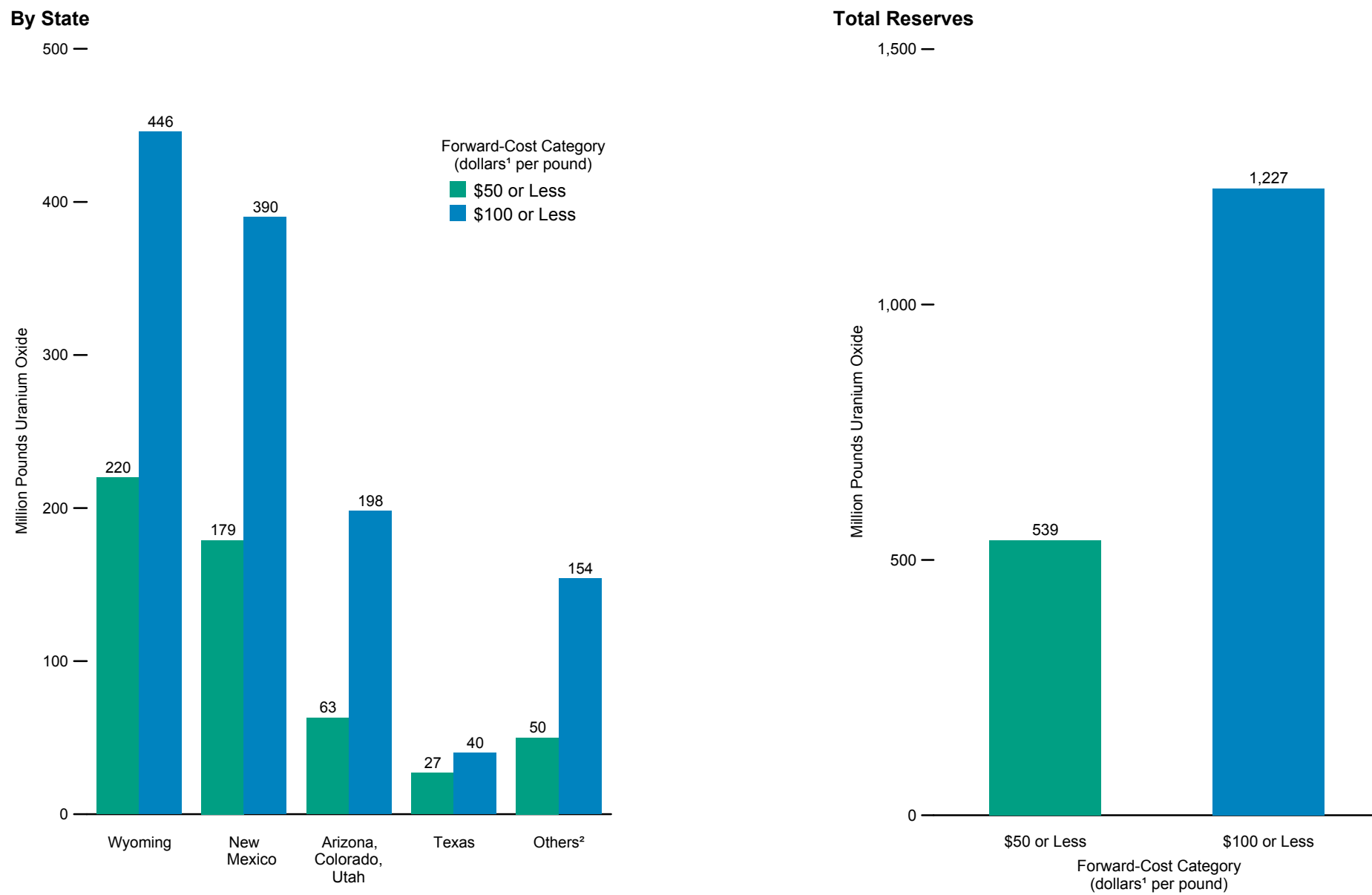
Figure 4.10 Uranium Reserves, 2008
