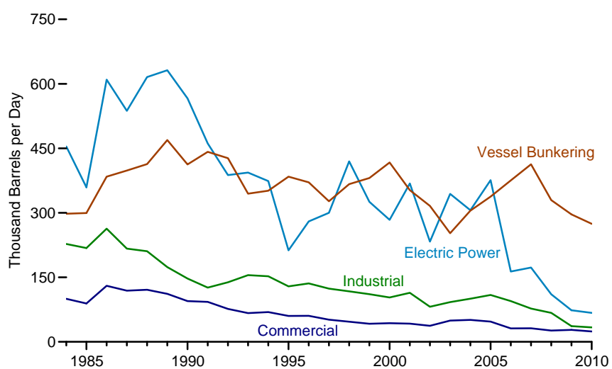
Residual Fuel Oil by Major End Use
