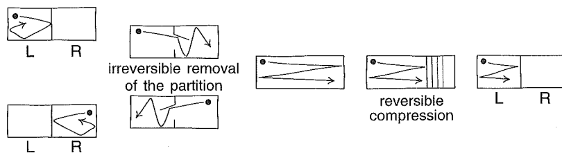
Fig. 2. The erasure process.
