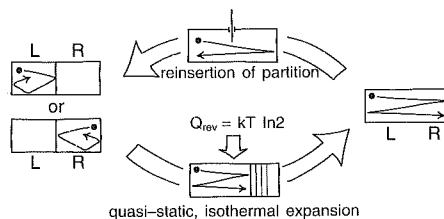
Fig. 5. Thermodynamic entropy no longer a state function with redefined notion of thermodynamic reversibility.
