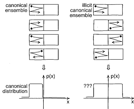
Fig. 3. Licit and illicit canonical ensembles and the distributions they produce.
