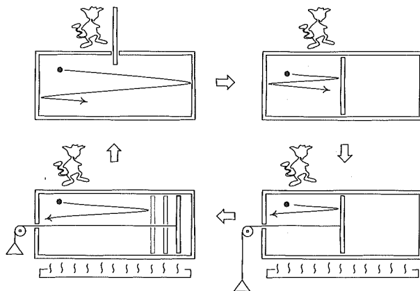
Fig. 7. Maxwell's demon operates Szilard's one-molecule gas engine.
