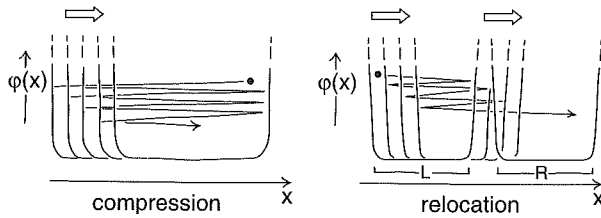
Fig. 1. Thermodynamically reversible processes due to slow change in potential field.
