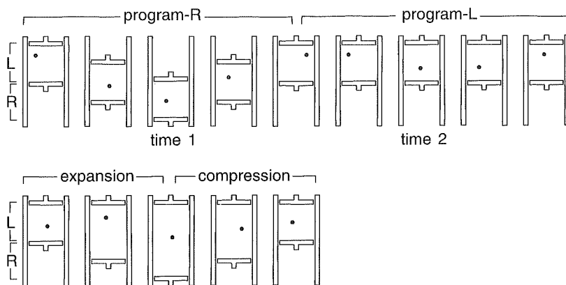
Fig. 8. Time development of the no-erasure demon's memory device and a different device that expands and contracts the phase space.
