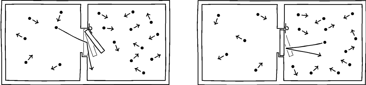
Figure 4 Smoluchowski Trapdoor
