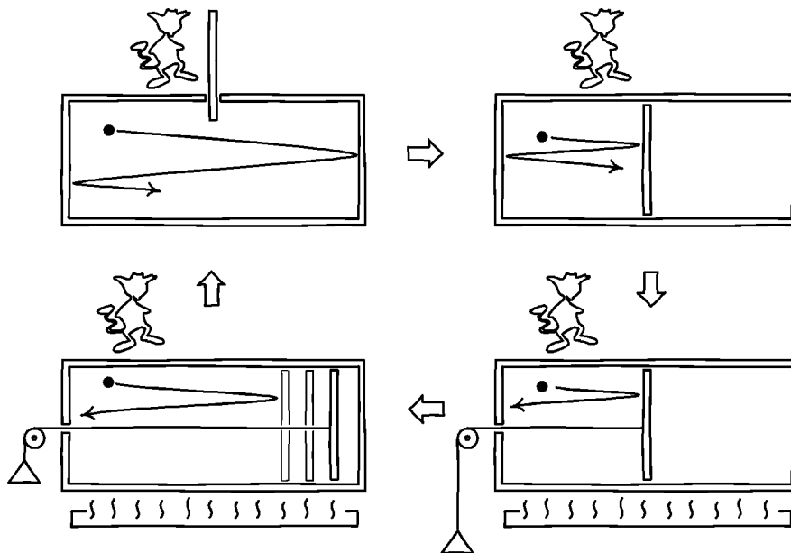
Figure 5. Maxwell's demon operates Szilard's one molecule gas engine
