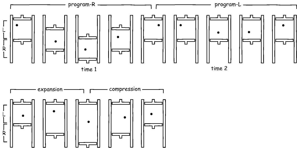
Figure 6 Time development of the no erasure demon's memory device and a different device that expands and contracts the phase space
