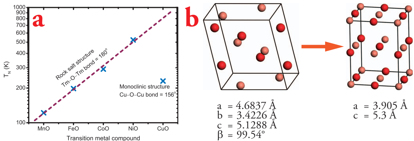
FIG. 1. (Color) (a) An overview of the Néel temperatures for transition metal monoxides with a rocksalt structure. T_N increases exponentially with each element up to NiO as indicated by the dashed line, which is a fit of the first four points. The T_N of the monoclinic CuO structure does not follow this trend, but is much lower, possibly due to a change in the Tm-O-Tm bond angle. When a rocksalt structure of CuO is formed, T_N might follow the trend and linear extrapolation predicts a T_N slightly higher than 800 K. (b) The change in unit-cell symmetry going from bulk (monoclinic) to the strained unit cell on SrTiO 3 (tetragonal), including the unit-cell parameters. The lighter colored atoms represent oxygen and the darker colored atoms represent copper.
