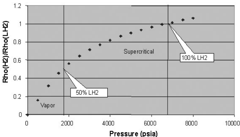
FIGURE 3. Mass density of gaseous hydrogen relative to the liquid state as a function of pressure. Those pressures at which the mass density is equivalent to 50% (1850 psia) and 100% (6800 psia) of liquid hydrogen are flagged.
