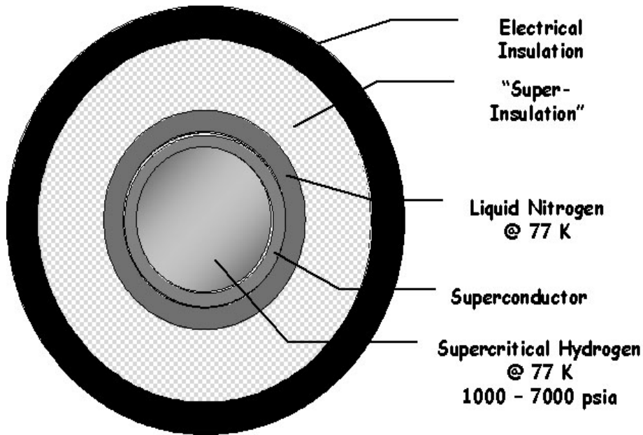
FIGURE 4. Hydricity SuperCable configuration employing gaseous hydrogen in the supercritical state at 77 K and high pressure. Here the pressurized hydrogen gas is surrounded by a shell of liquid nitrogen which is the principal cryogen.
