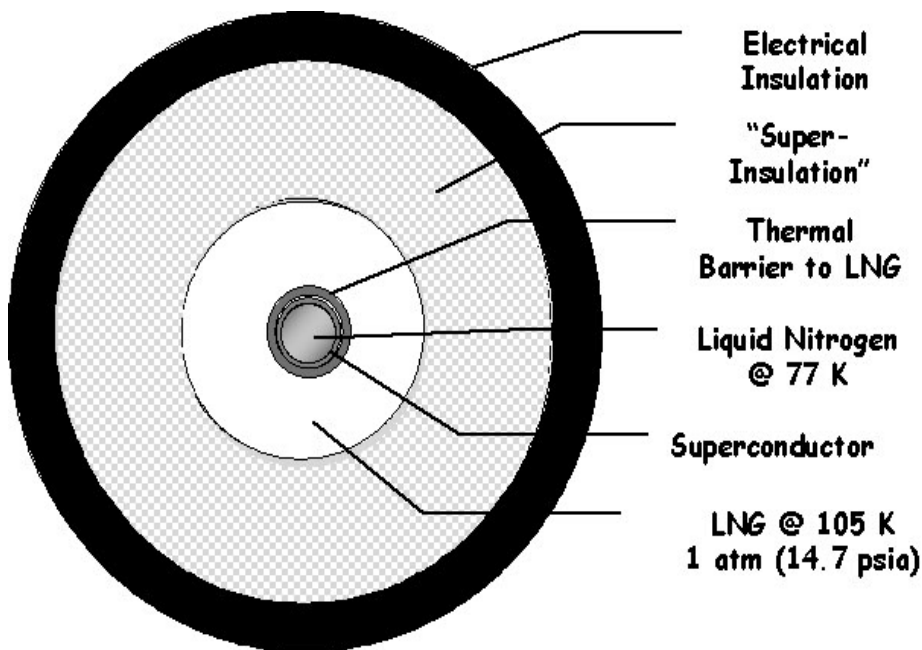
FIGURE 6. Monopole cross-section of a conceptual Liquidified Natural Gas SuperCable. The cryogen is liquid nitrogen flowing through the center cylindrical tube. Note the presence of a heat shield between the superconductor layer and the LNG channel in order to keep its temperature above 86 K, the freezing point of methane.
