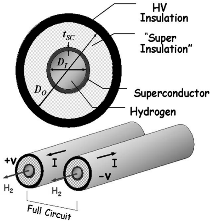
FIGURE 2. Schematic of a possible Hydricity SuperCable configuration consisting of a bipolar superconducting dc electrical circuit cooled by liquid hydrogen. The upper diagram depicts the cross-section of one monopole. The superconducting component, shown as an annulus in the diagram, can in fact be of rather arbitrary diameter as long as it remains immersed in the hydrogen cryofluid.
